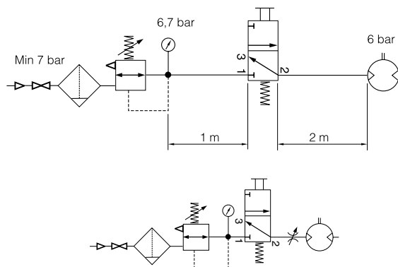
Shut-off, filtering, pressure regulation and control valve
